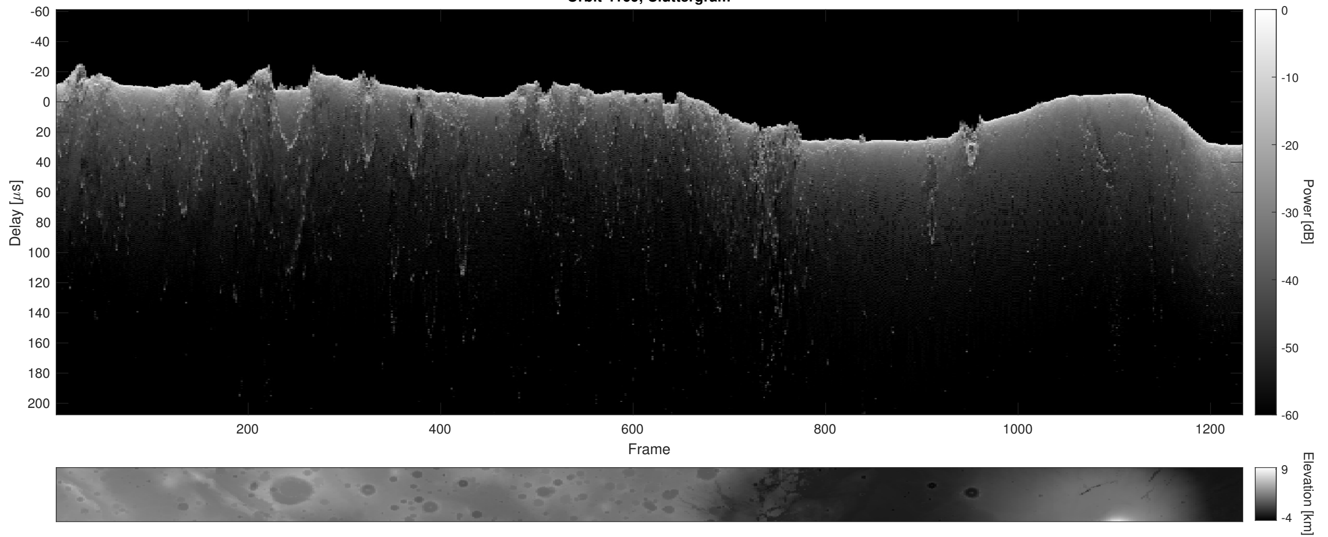
Orbit 4169, Cluttergram
