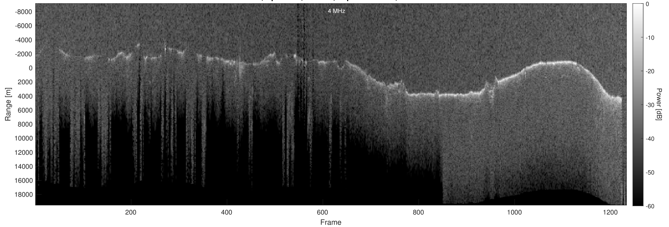
Orbit 4169, Optimized, Window, Depth-Corrected, Channel 2
