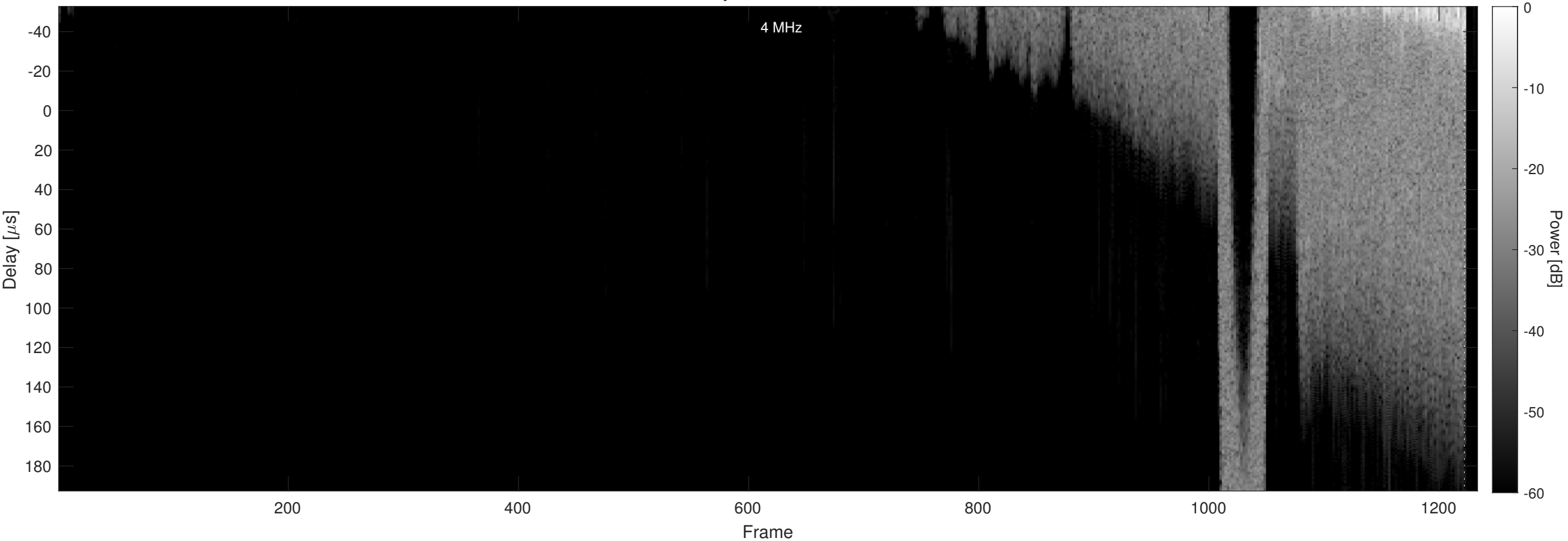
Orbit 4170, Chapman, Window, Channel 2
