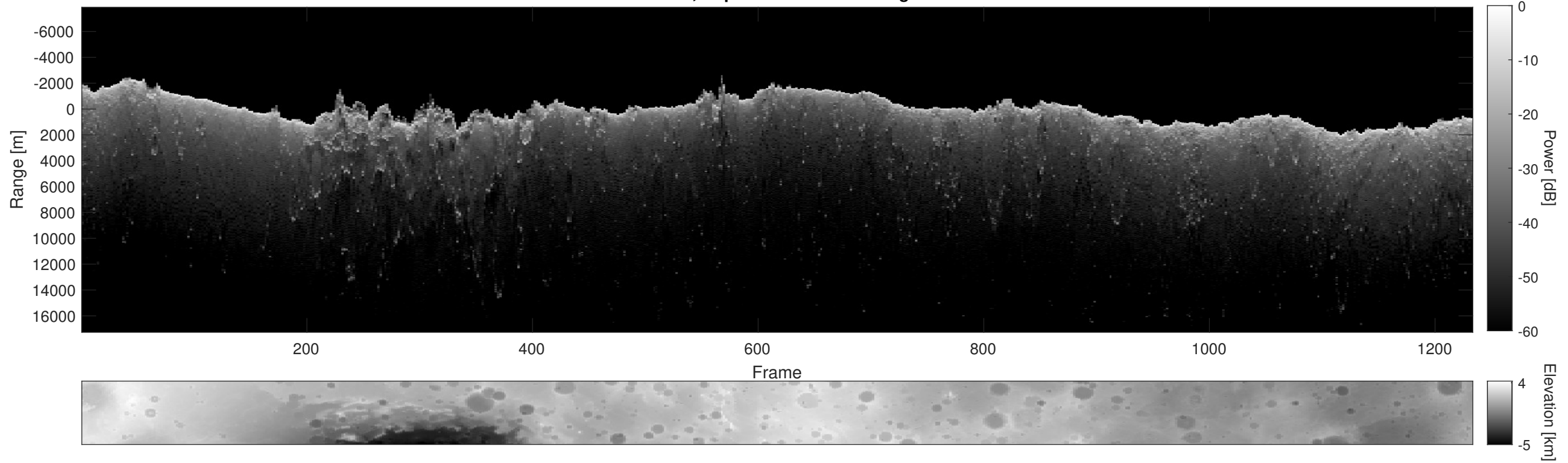
Orbit 4170, Depth-Corrected Cluttergram
