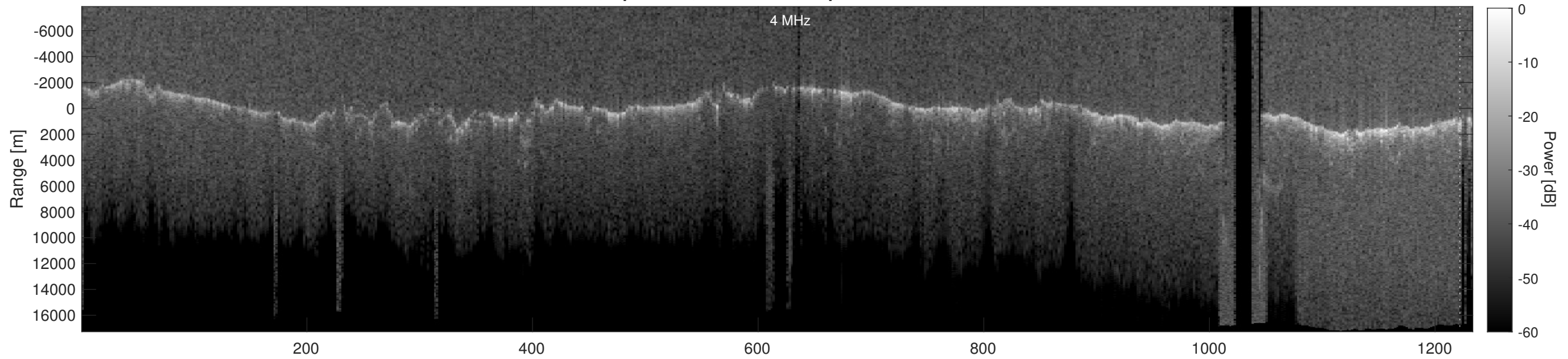
Orbit 4170, Depth-Corrected Cluttergram
