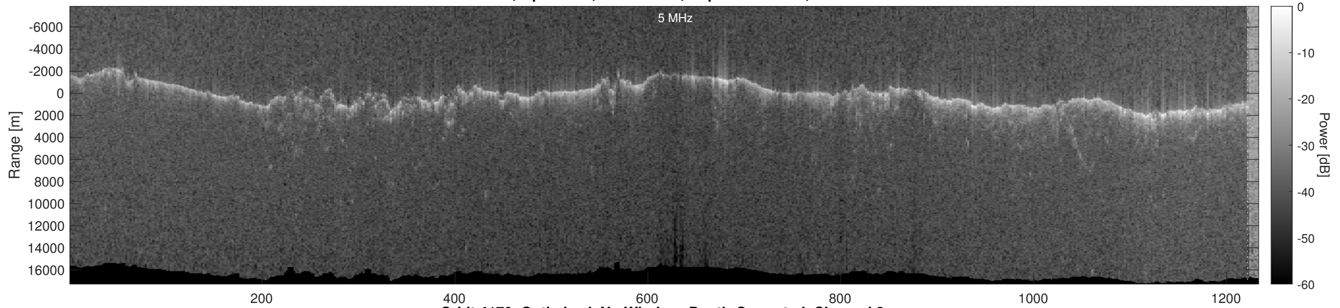
Orbit 4170, Optimized, No Window, Depth-Corrected, Channel 2
