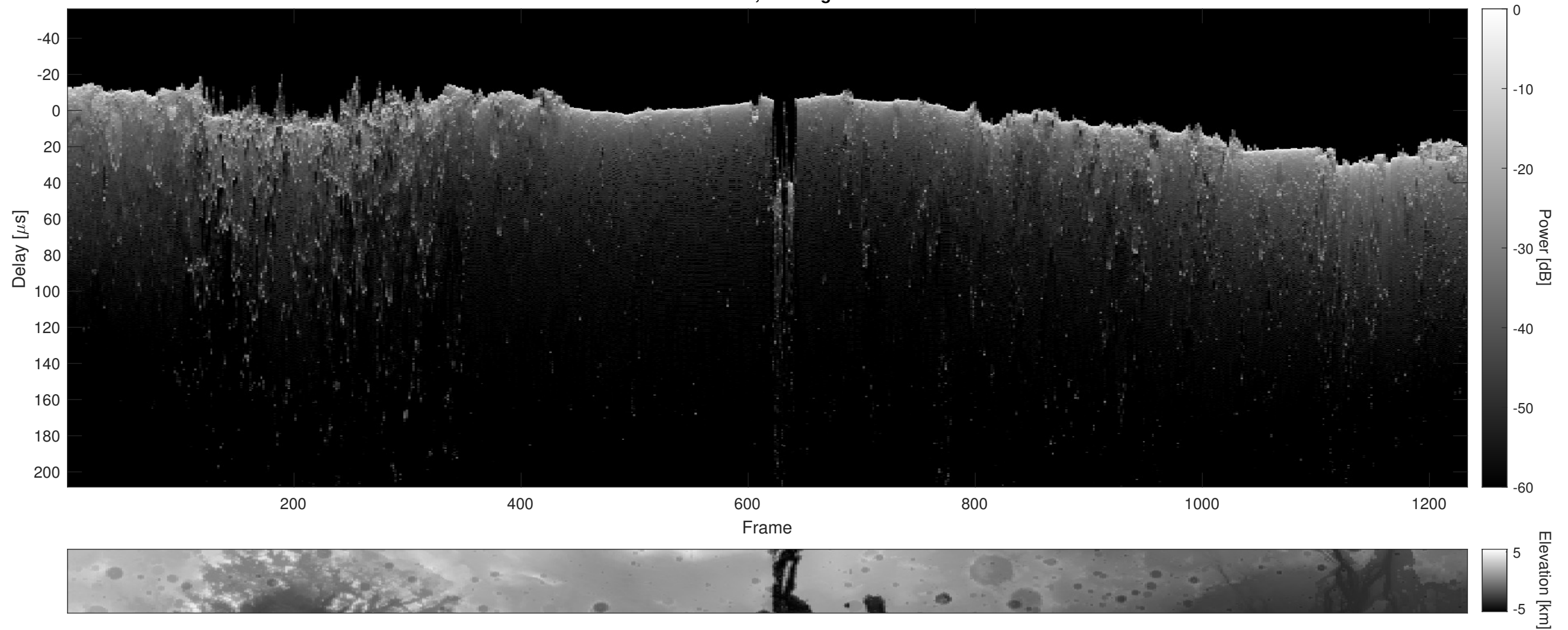
Orbit 4171, Cluttergram
