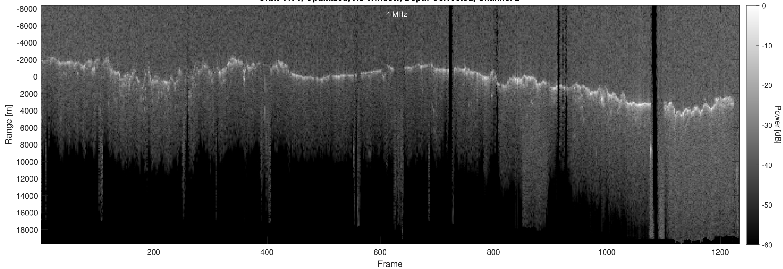
Orbit 4171, Optimized, No Window, Depth-Corrected, Channel 2
