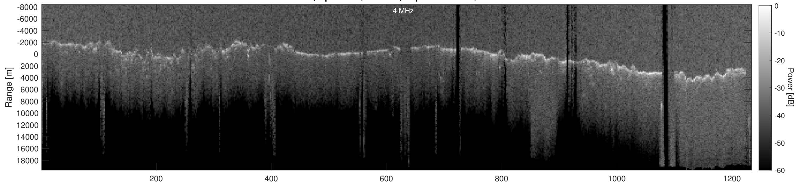
Orbit 4171, Depth-Corrected Cluttergram
