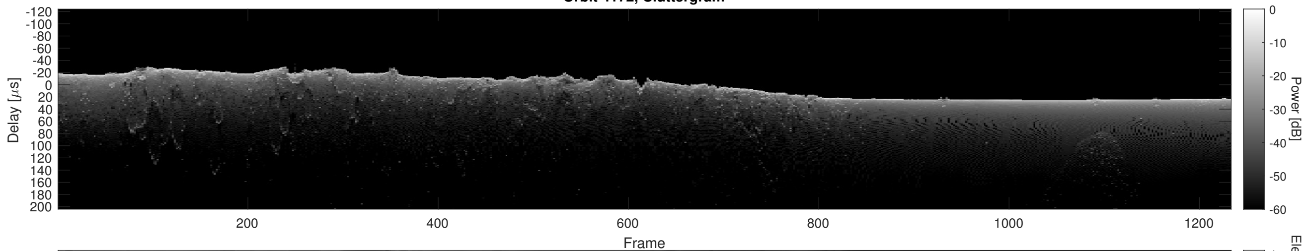
Orbit 4172, Cluttergram
