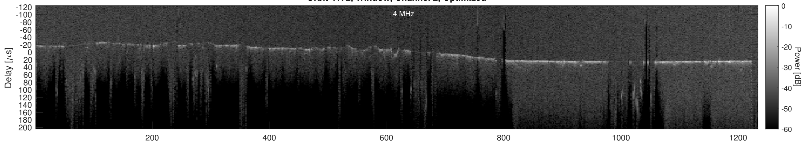
Orbit 4172, Cluttergram
