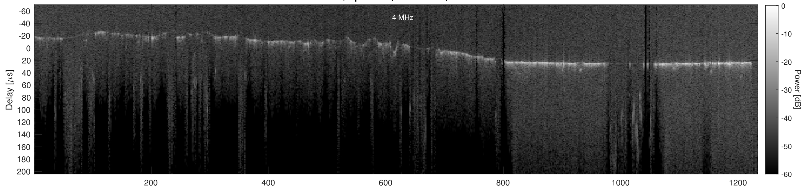
Orbit 4172, Cluttergram
