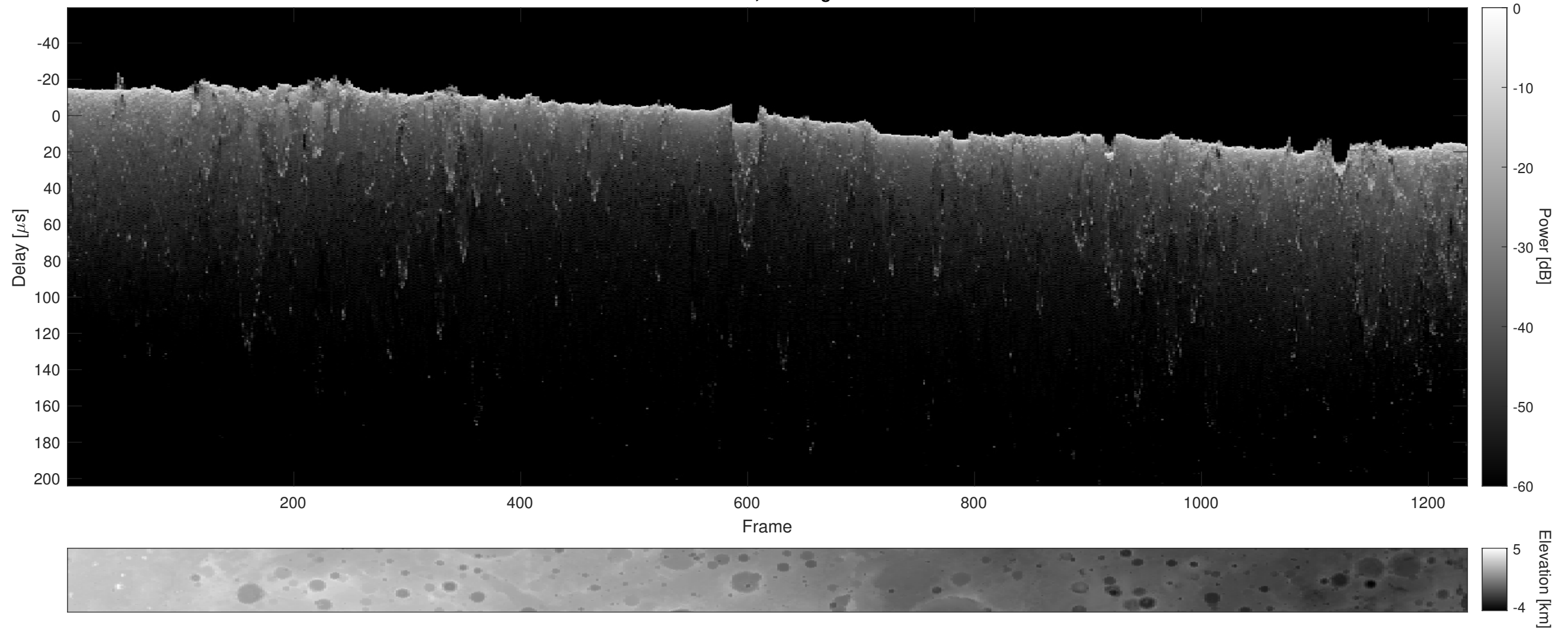
Orbit 4174, Cluttergram
