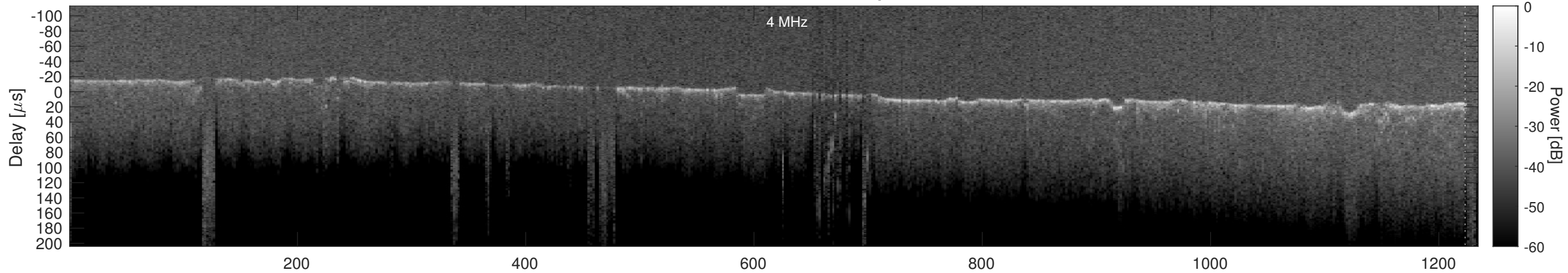
Orbit 4174, Cluttergram
