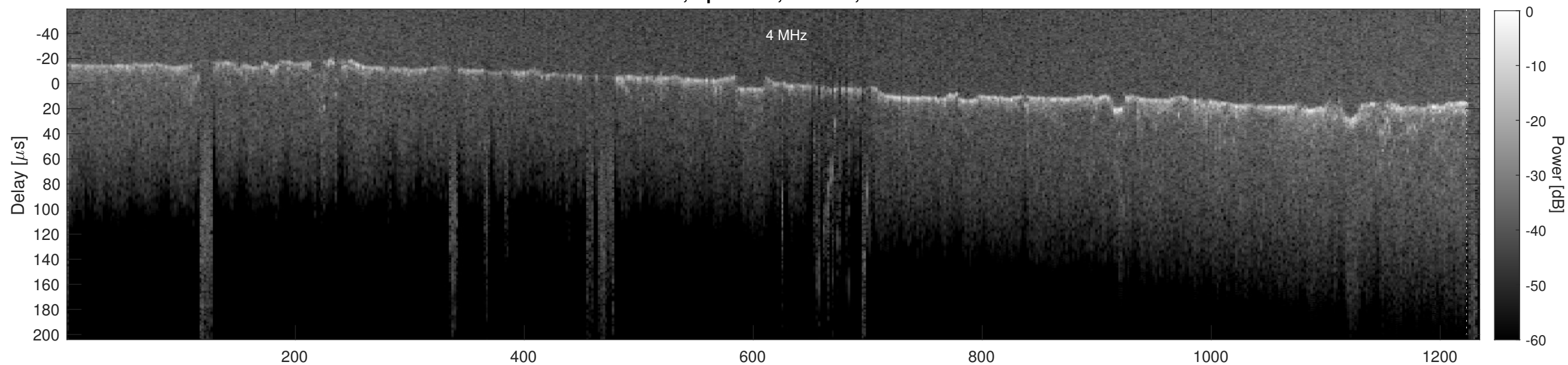
Orbit 4174, Cluttergram
