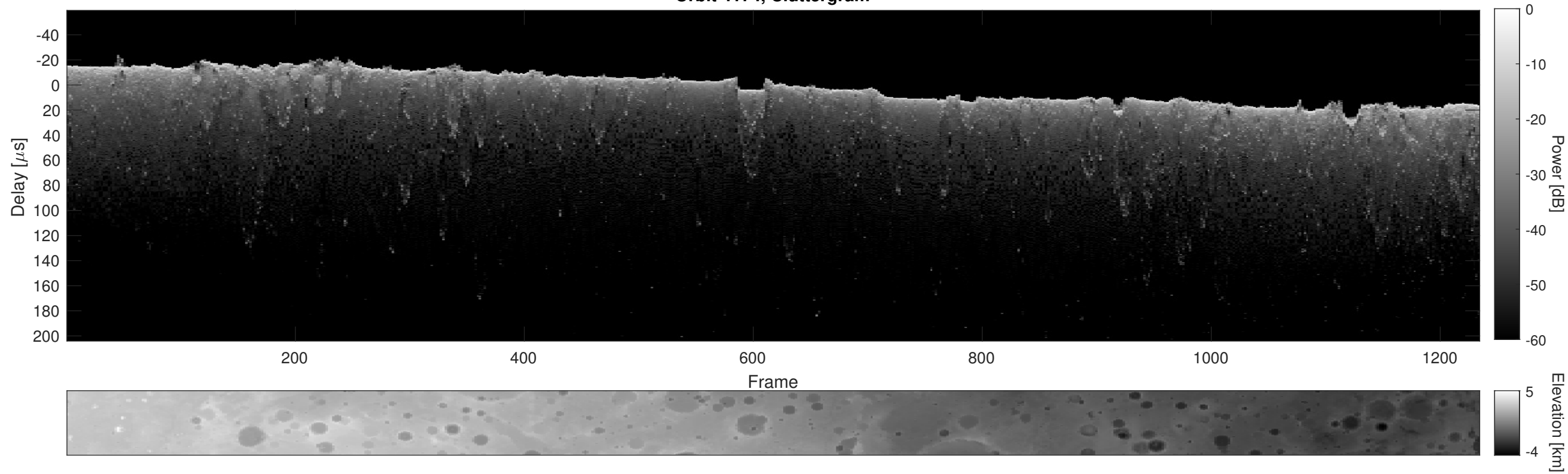
Orbit 4174, Cluttergram
