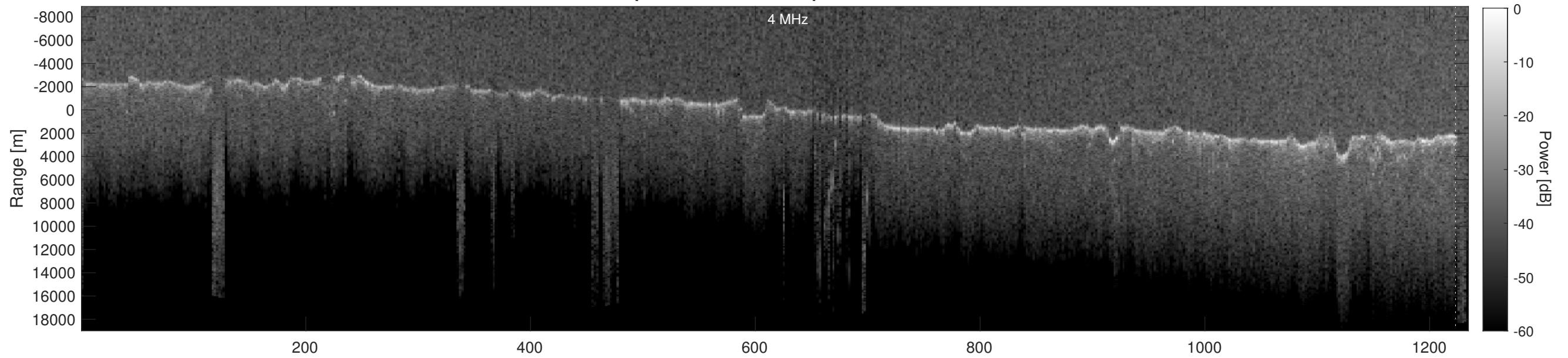
Orbit 4174, Depth-Corrected Cluttergram
