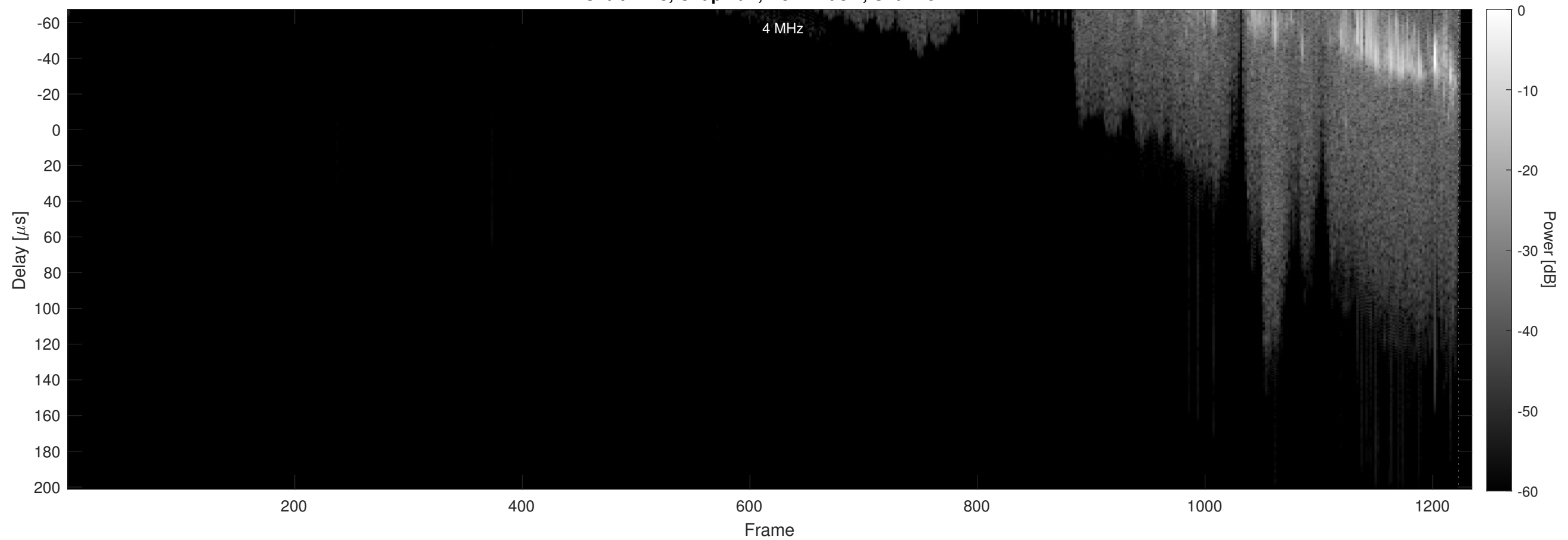
Orbit 4178, Chapman, No Window, Channel 2
