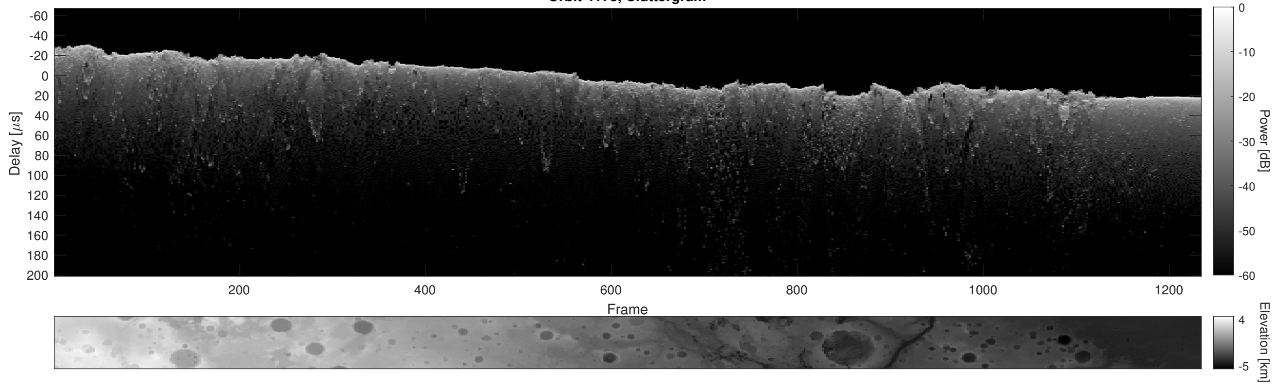
Orbit 4178, Cluttergram
