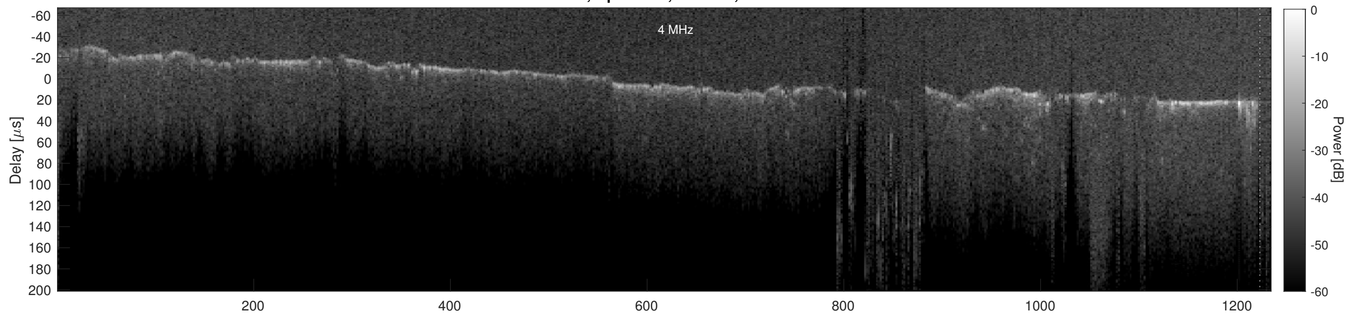
Orbit 4178, Cluttergram
