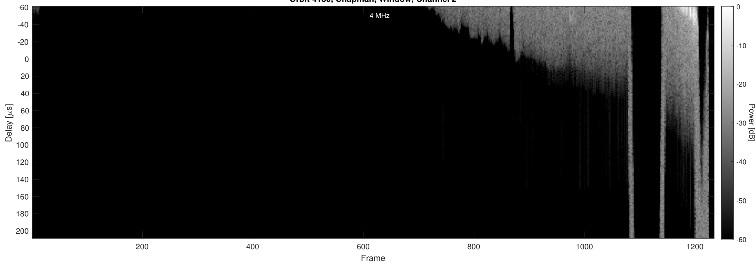
Orbit 4180, Chapman, Window, Channel 2
