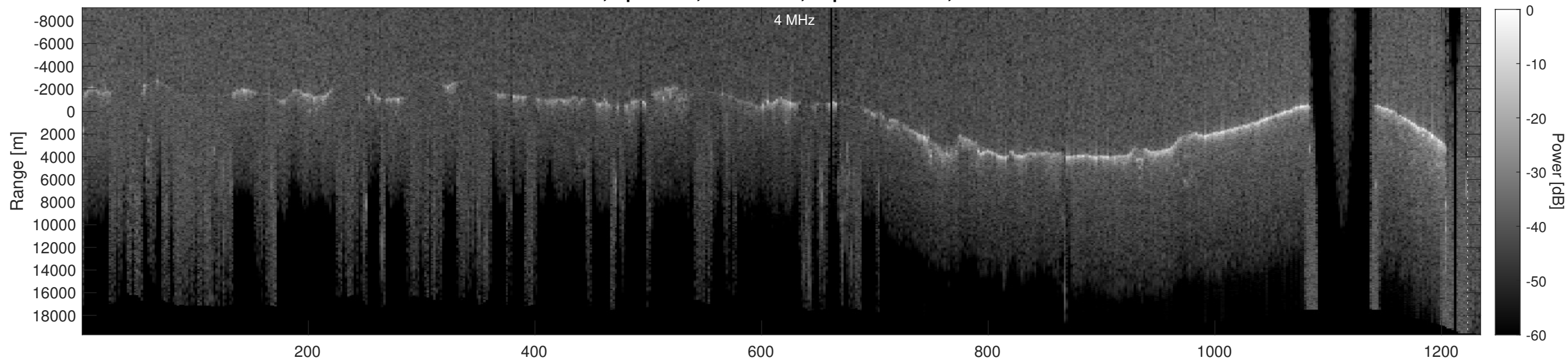
Orbit 4180, Depth-Corrected Cluttergram
