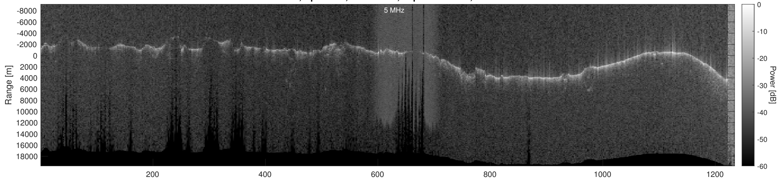
Orbit 4180, Optimized, No Window, Depth-Corrected, Channel 2
