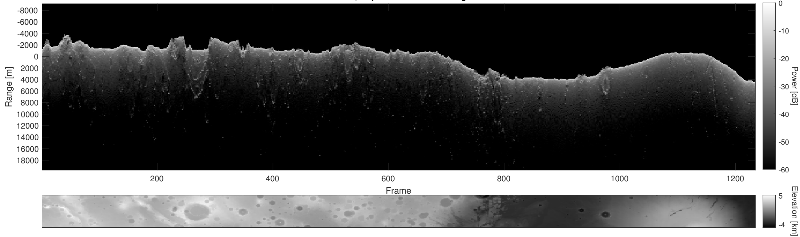
Orbit 4180, Depth-Corrected Cluttergram
