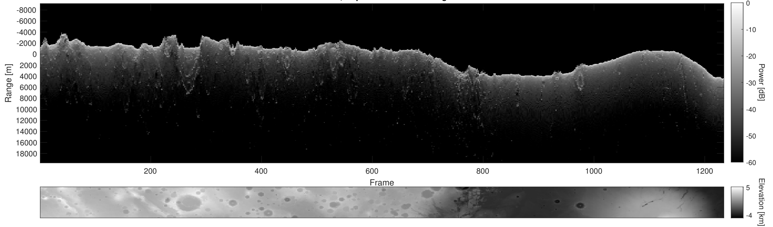
Orbit 4180, Depth-Corrected Cluttergram
