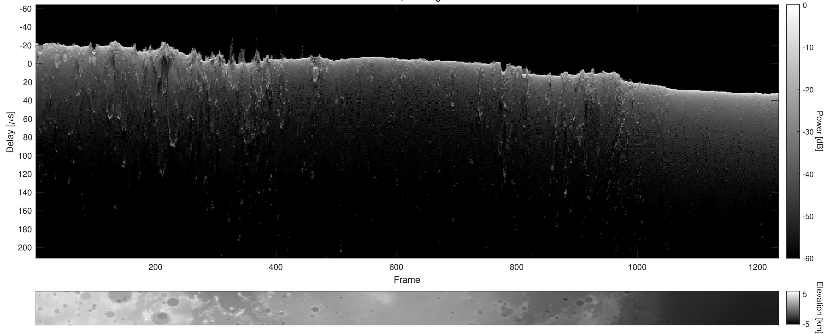
Orbit 4184, Cluttergram
