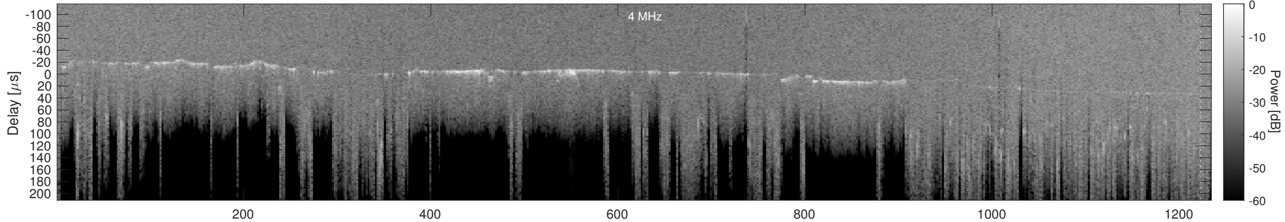
Orbit 4184, Cluttergram
