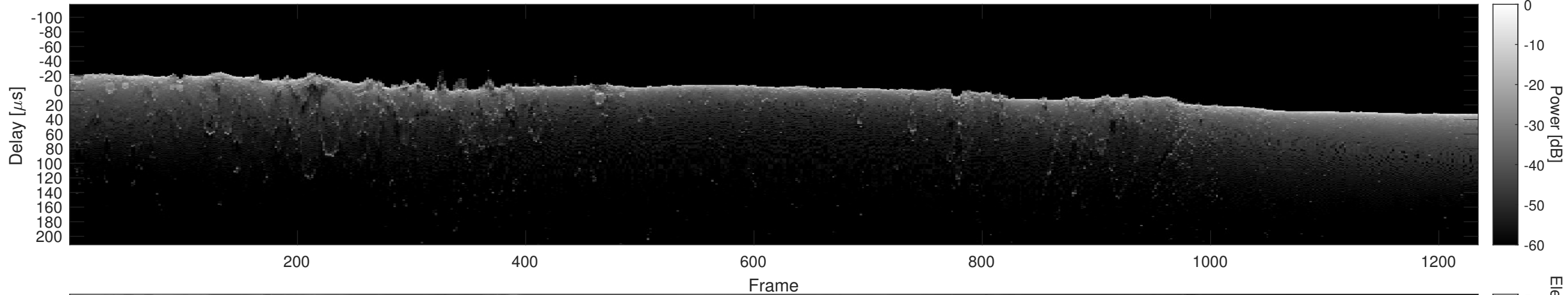
Orbit 4184, Cluttergram
