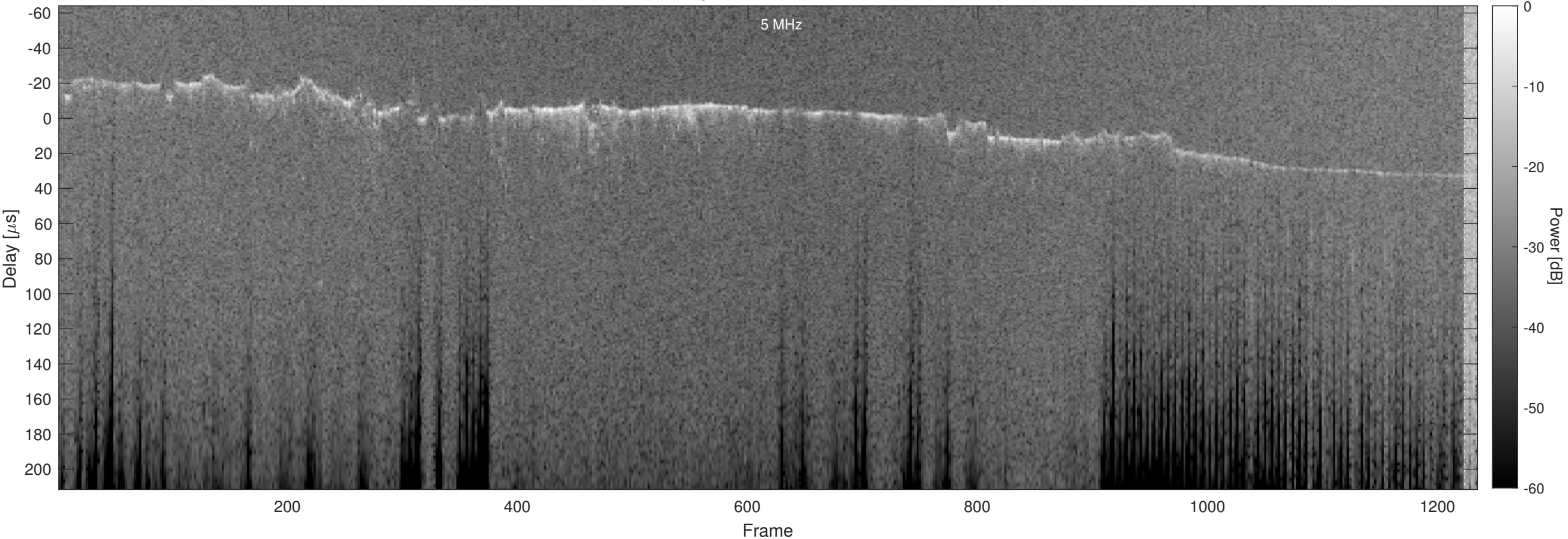
Orbit 4184, Optimized, Window, Channel 2
