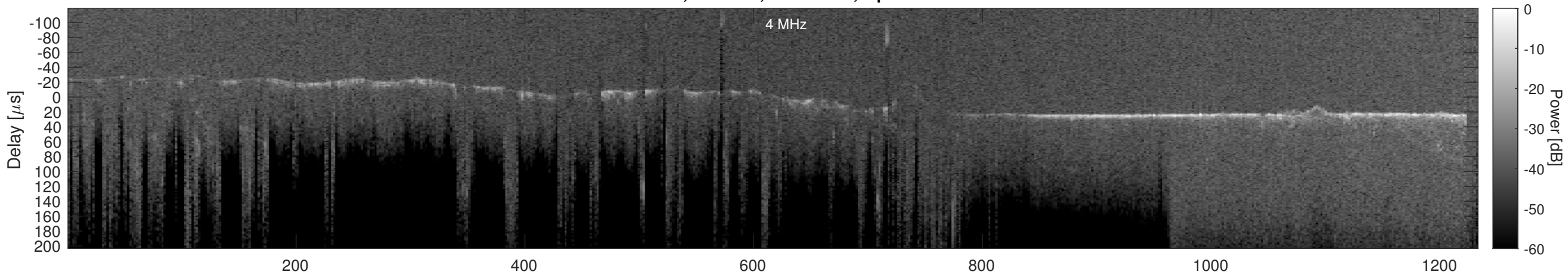
Orbit 4187, Cluttergram
