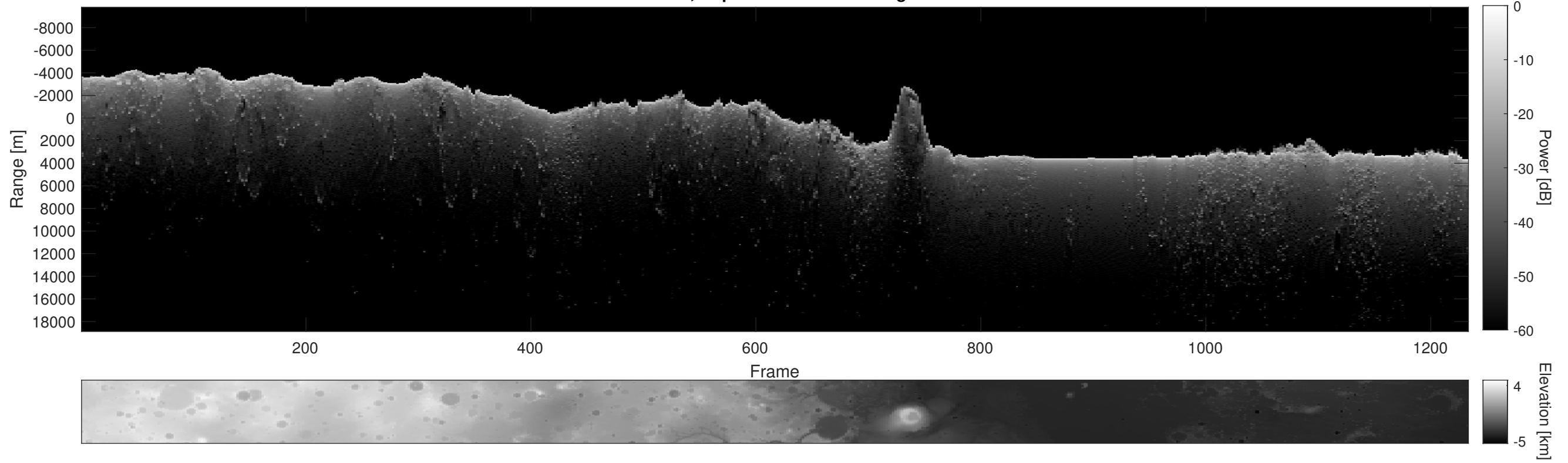
Orbit 4187, Depth-Corrected Cluttergram
