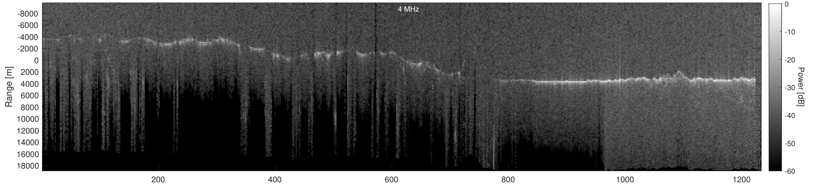
Orbit 4187, Depth-Corrected Cluttergram
