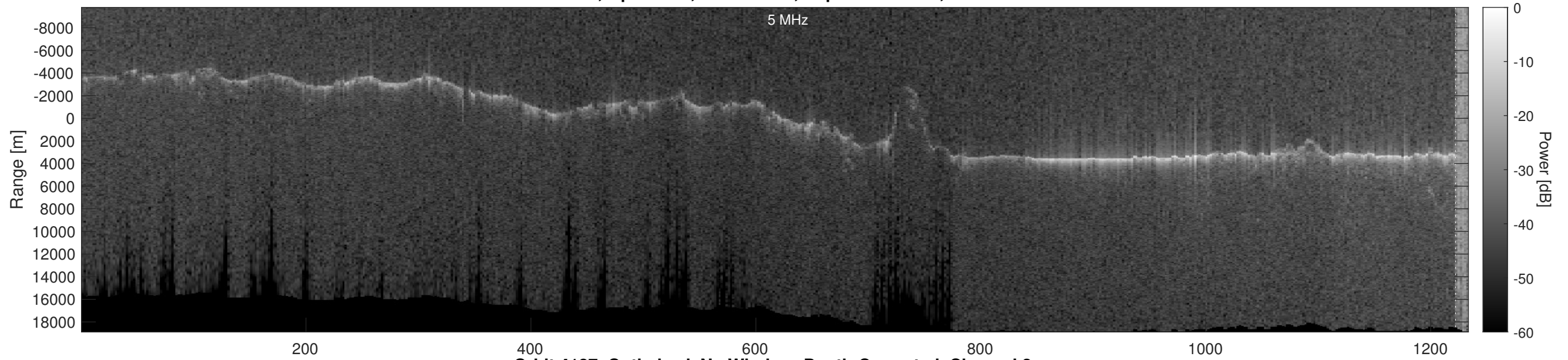
Orbit 4187, Optimized, No Window, Depth-Corrected, Channel 2
