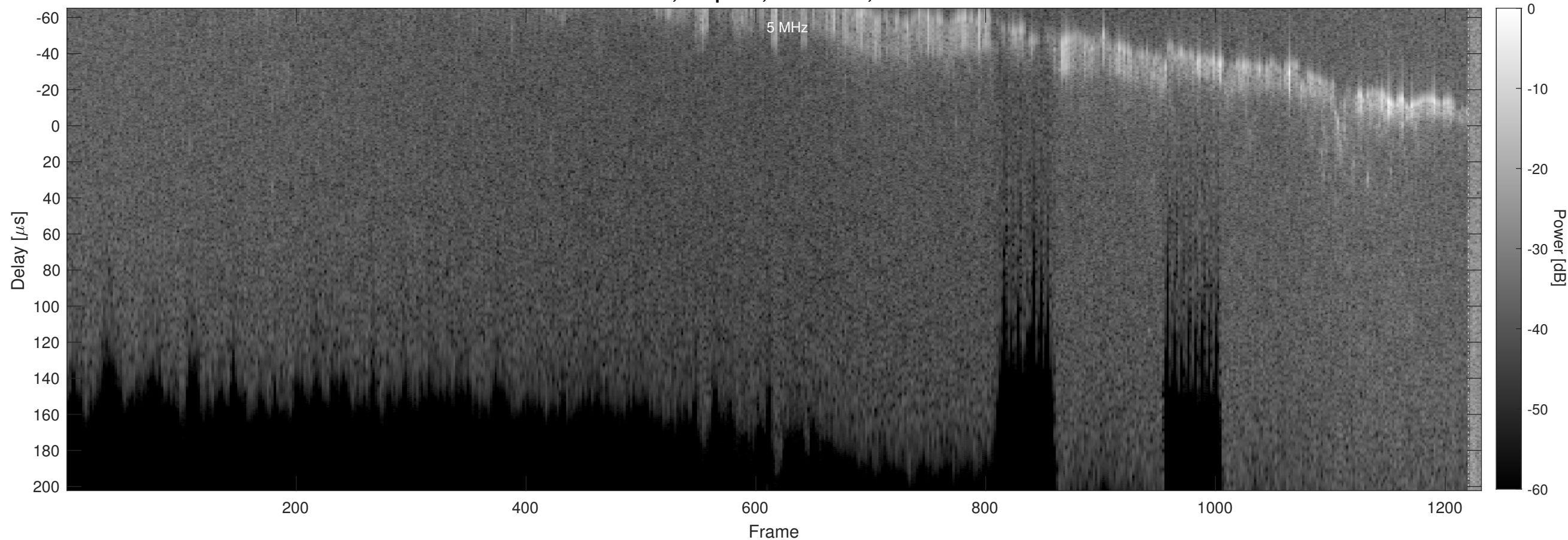
Orbit 4189, Chapman, No Window, Channel 2
