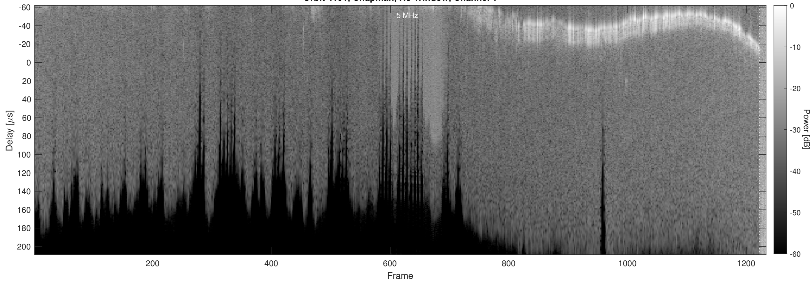
Orbit 4191, Chapman, No Window, Channel 2
