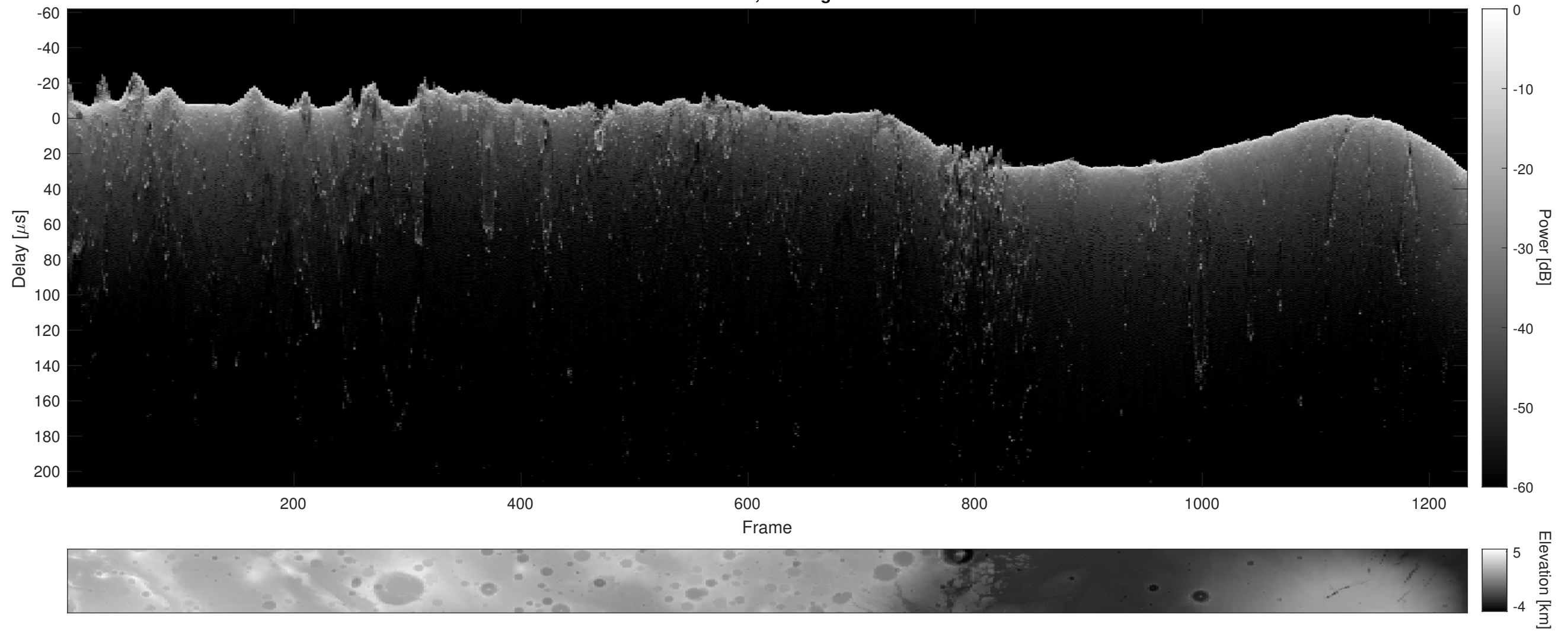
Orbit 4191, Cluttergram
