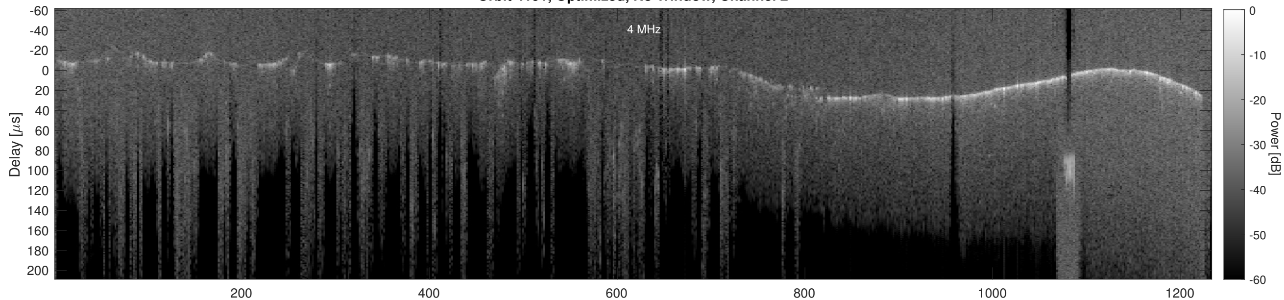
Orbit 4191, Cluttergram
