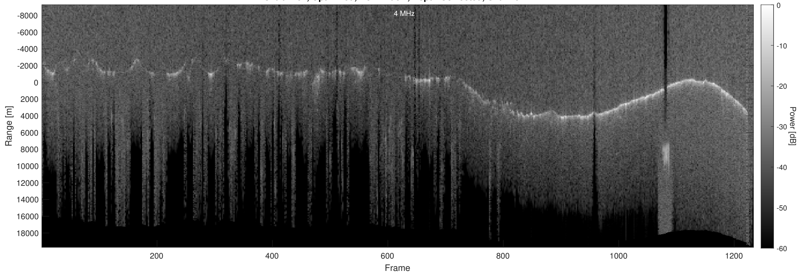
Orbit 4191, Optimized, No Window, Depth-Corrected, Channel 2
