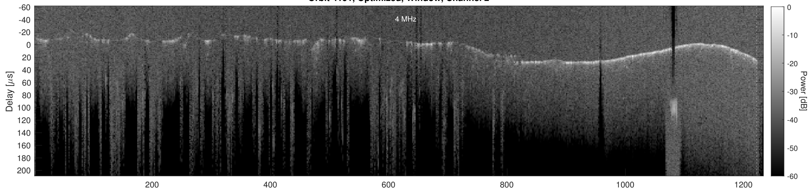
Orbit 4191, Cluttergram
