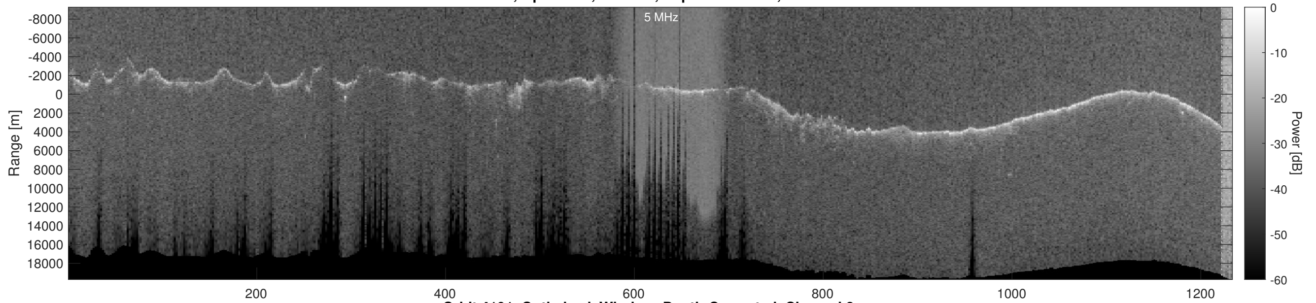
Orbit 4191, Optimized, Window, Depth-Corrected, Channel 2
