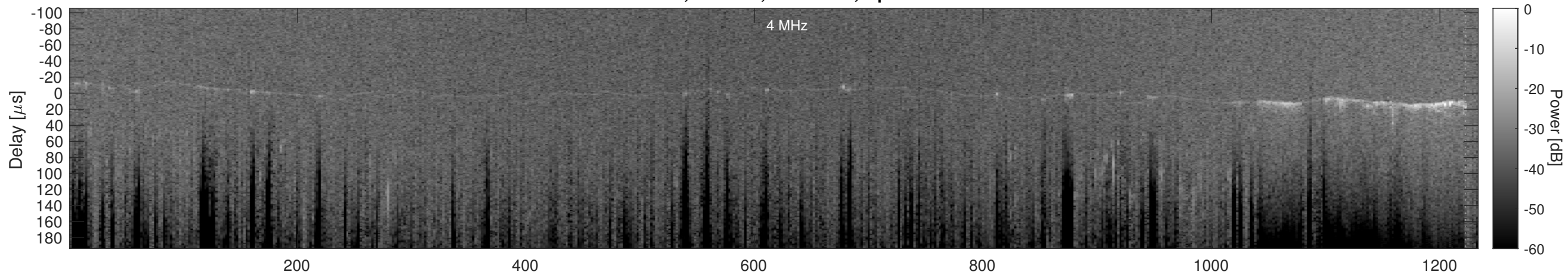
Orbit 4192, Cluttergram
