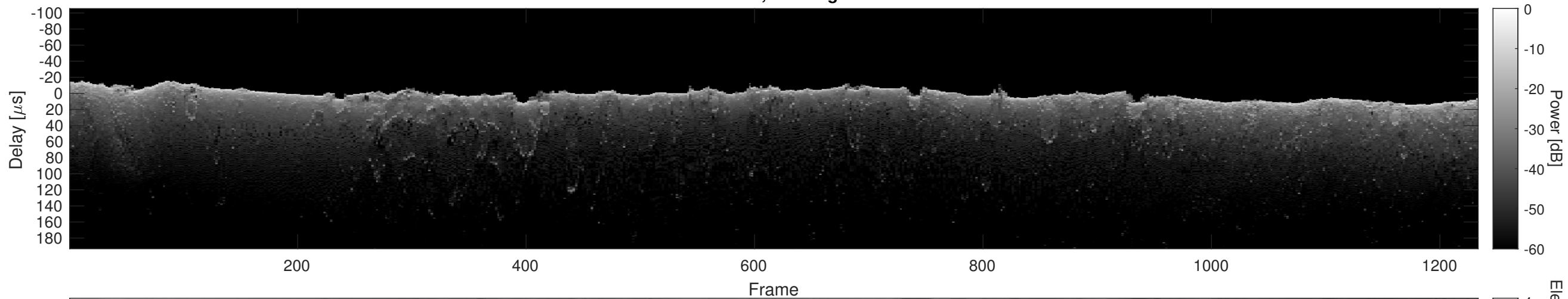
Orbit 4192, Cluttergram
