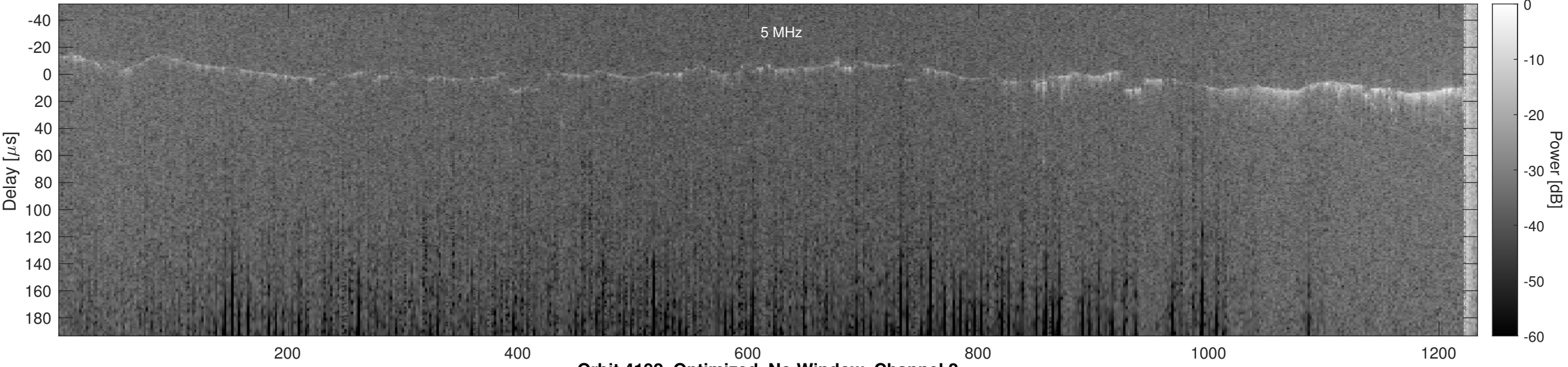
Orbit 4192, Optimized, No Window, Channel 2
