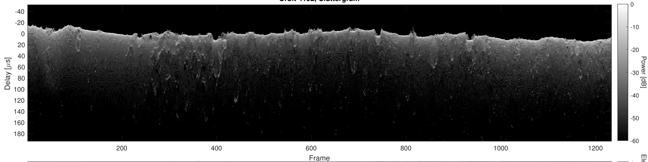
Orbit 4192, Cluttergram
