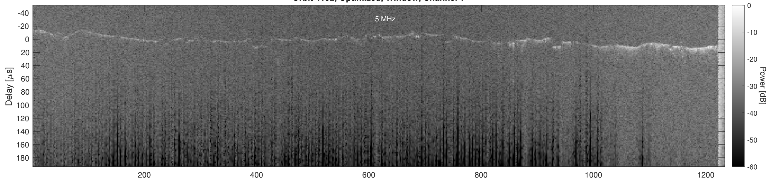
Orbit 4192, Optimized, Window, Channel 2
