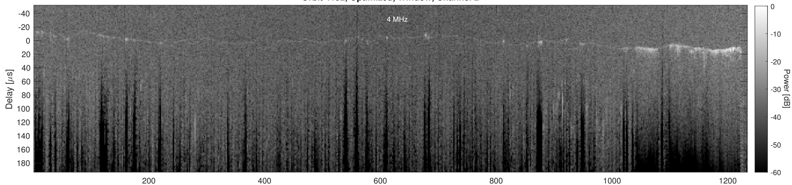
Orbit 4192, Cluttergram
