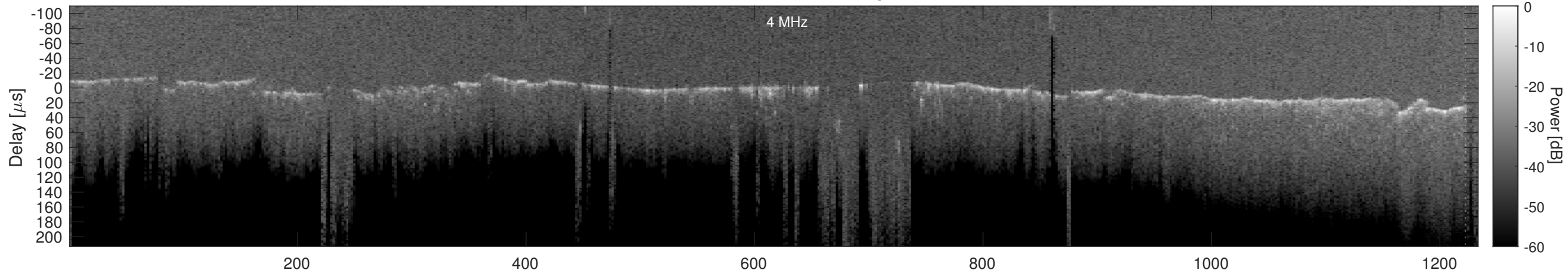
Orbit 4193, Cluttergram
