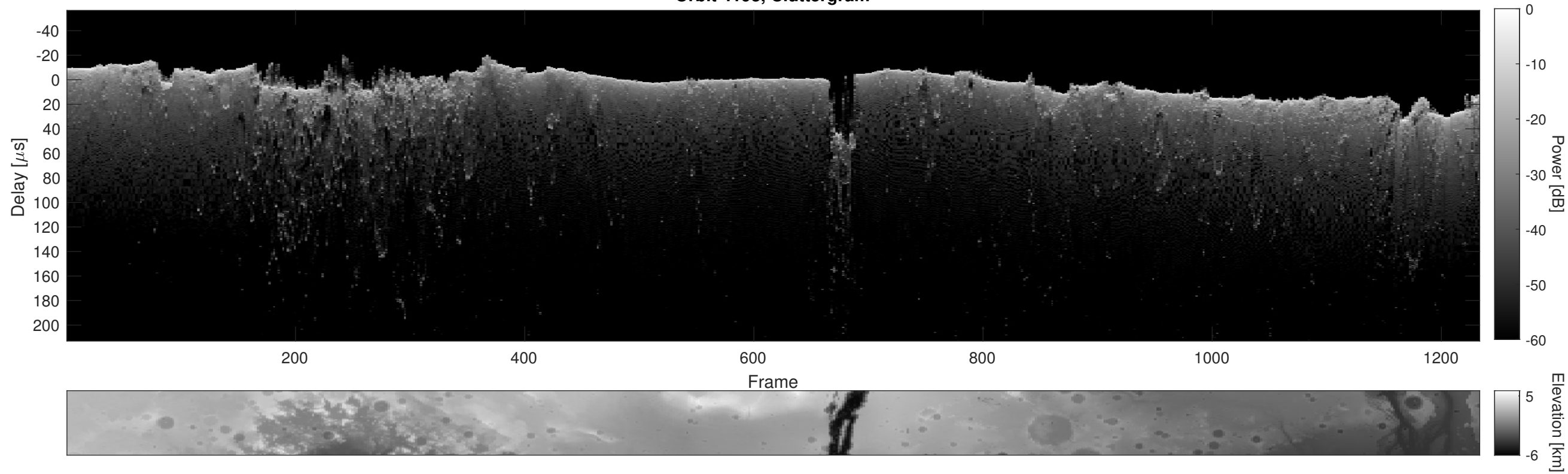
Orbit 4193, Cluttergram
