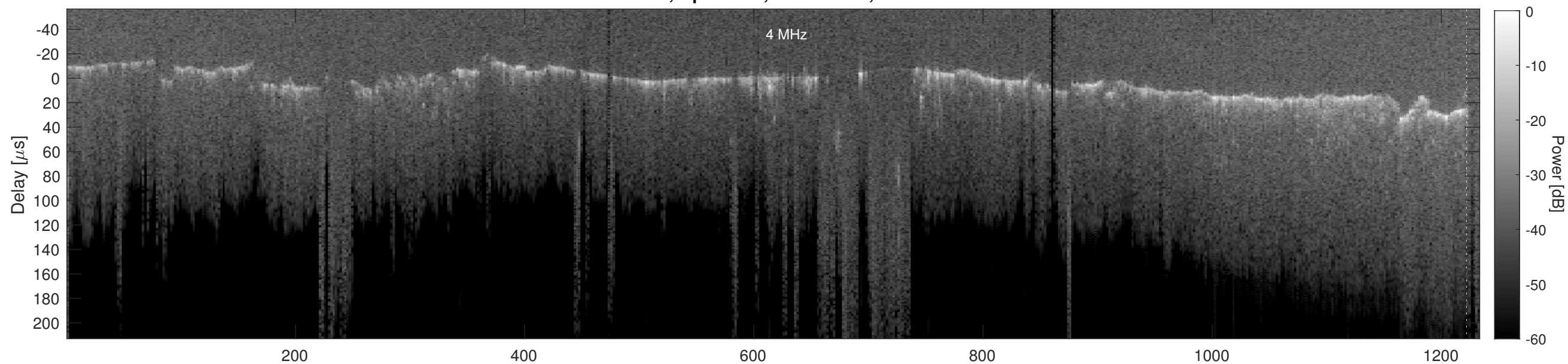
Orbit 4193, Cluttergram
