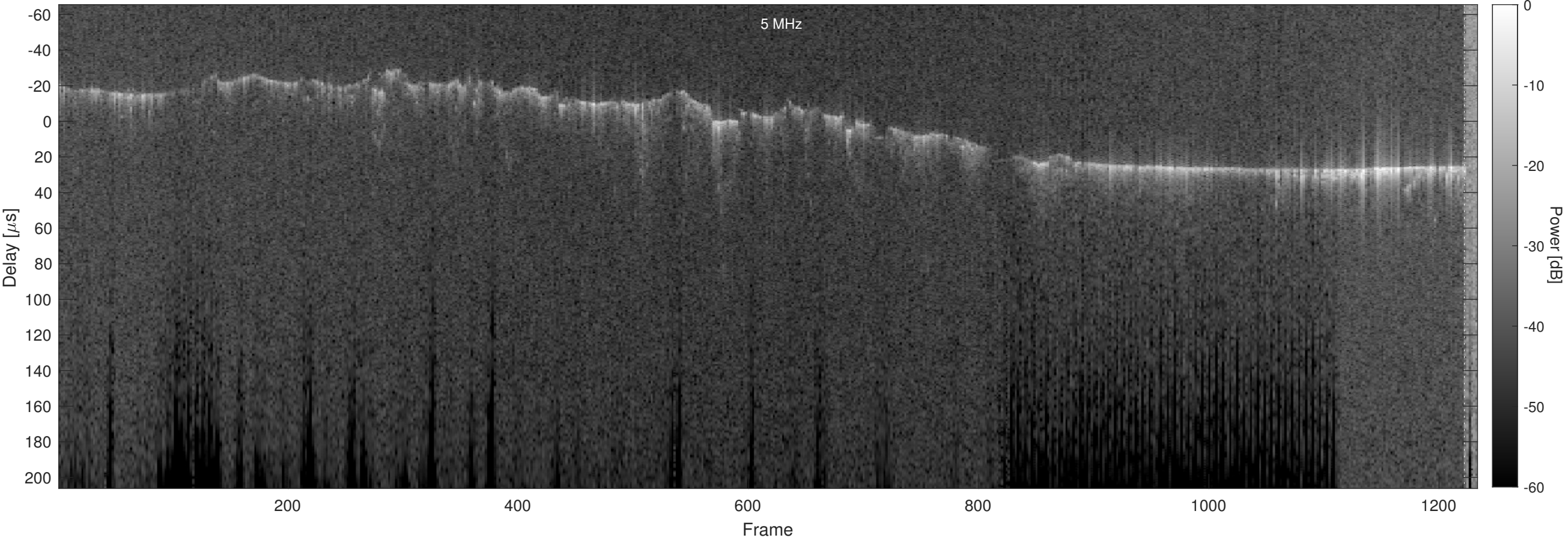
Orbit 4194, Optimized, No Window, Channel 2
