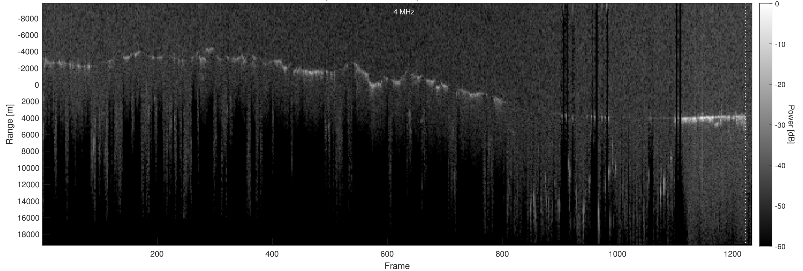
Orbit 4194, Optimized, Window, Depth-Corrected, Channel 2
