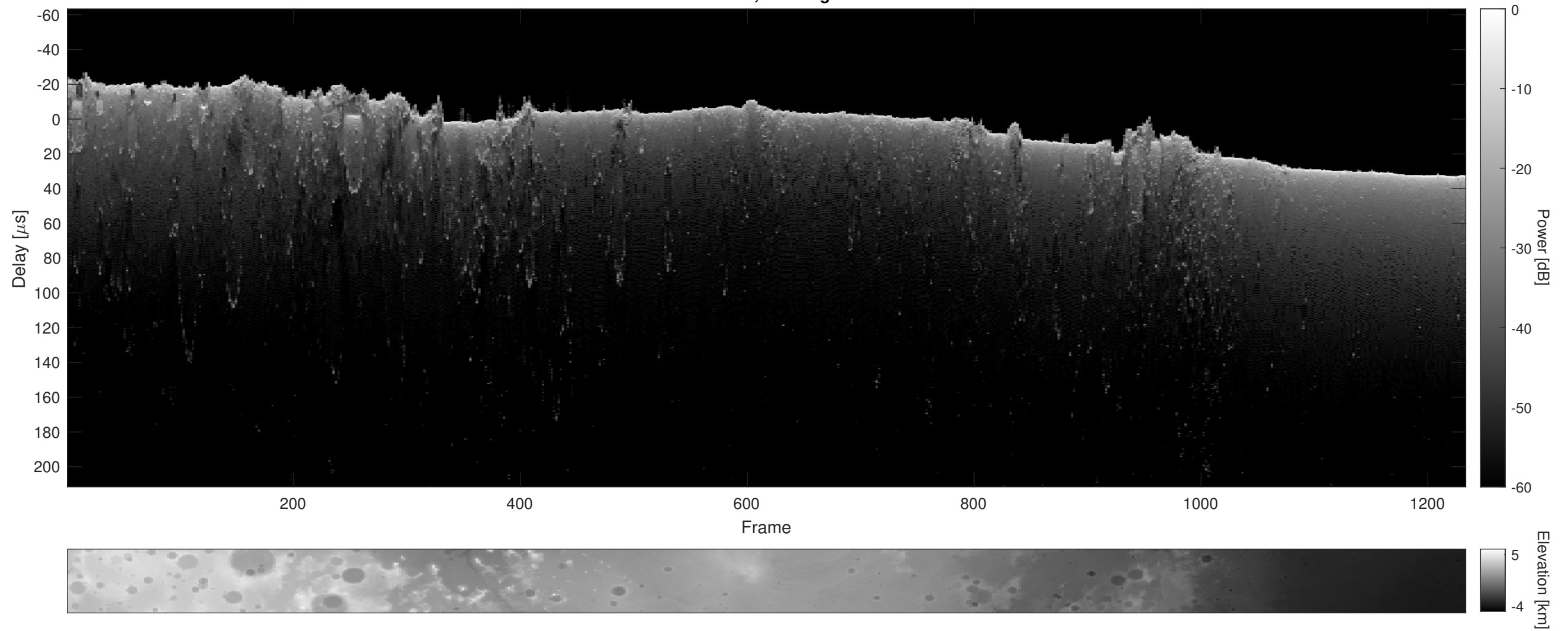
Orbit 4195, Cluttergram
