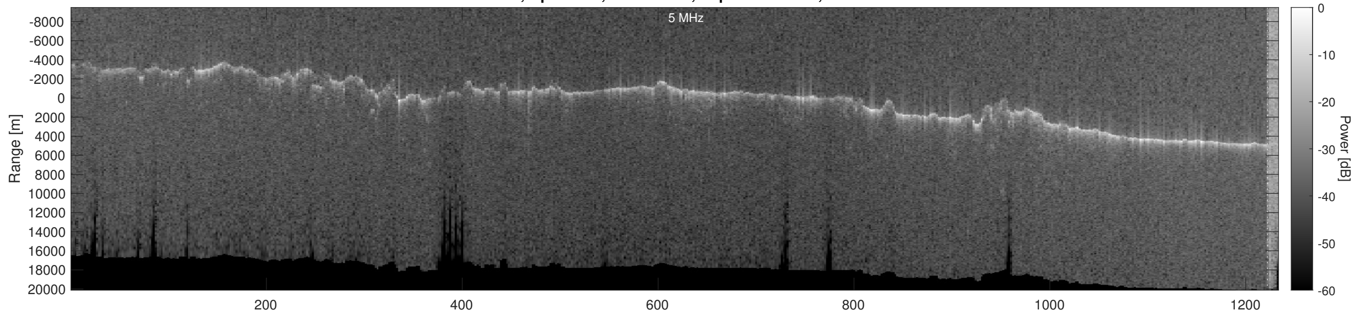
Orbit 4195, Optimized, No Window, Depth-Corrected, Channel 2
