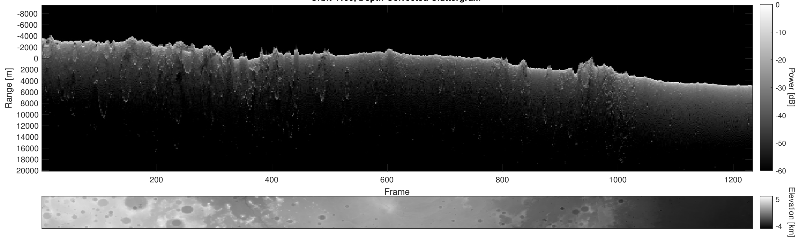
Orbit 4195, Depth-Corrected Cluttergram
