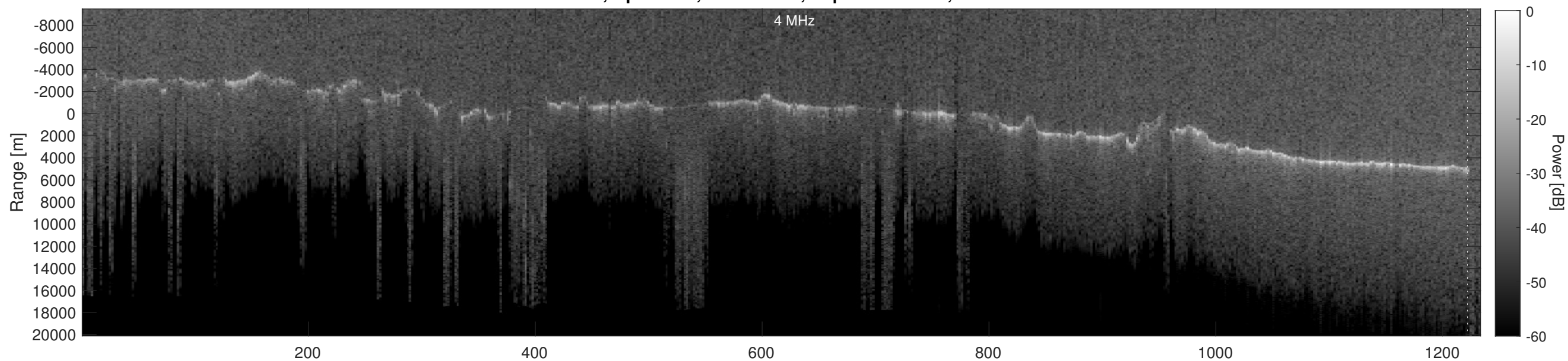
Orbit 4195, Depth-Corrected Cluttergram
