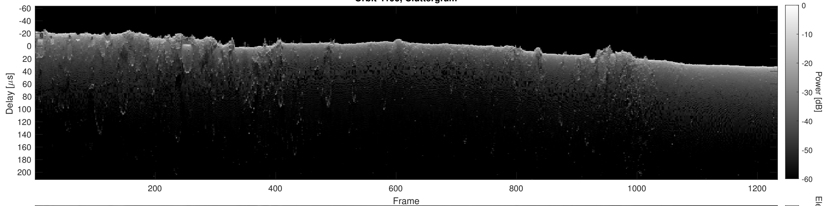
Orbit 4195, Cluttergram
