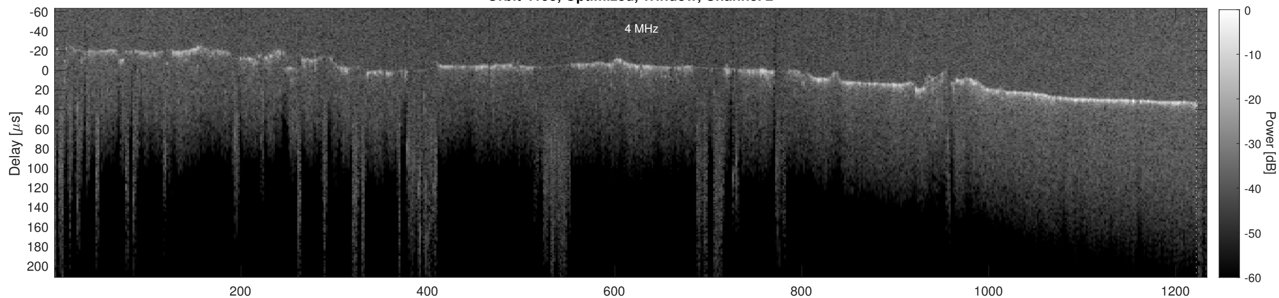
Orbit 4195, Cluttergram
