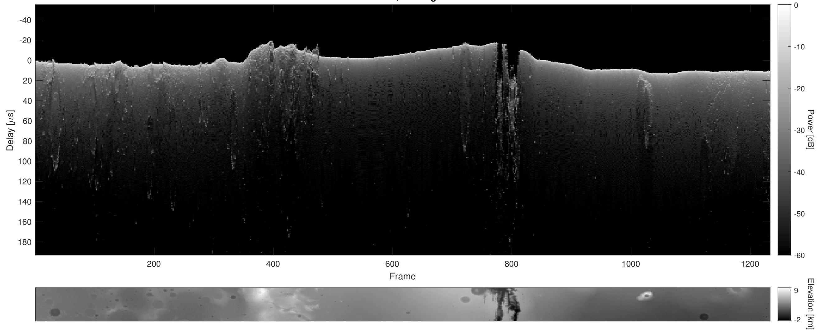
Orbit 4197, Cluttergram
