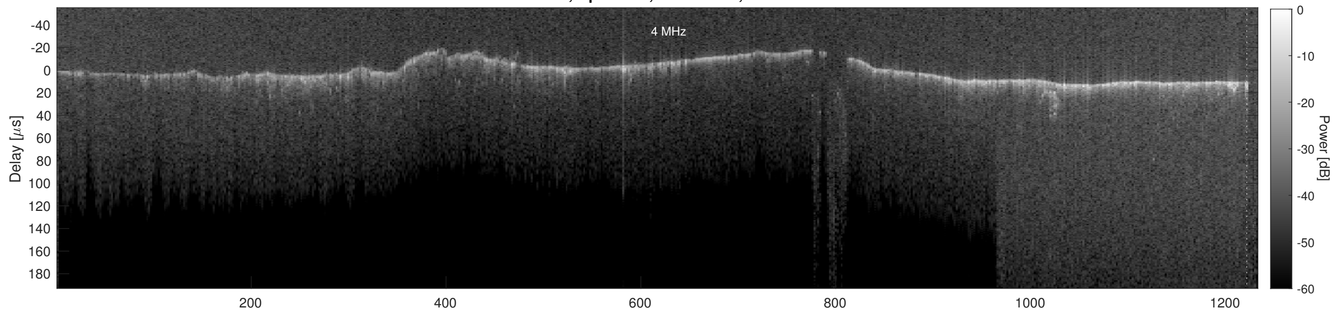
Orbit 4197, Cluttergram
