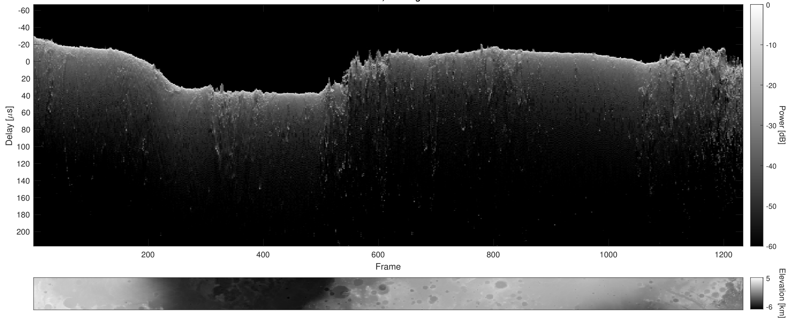
Orbit 4199, Cluttergram
