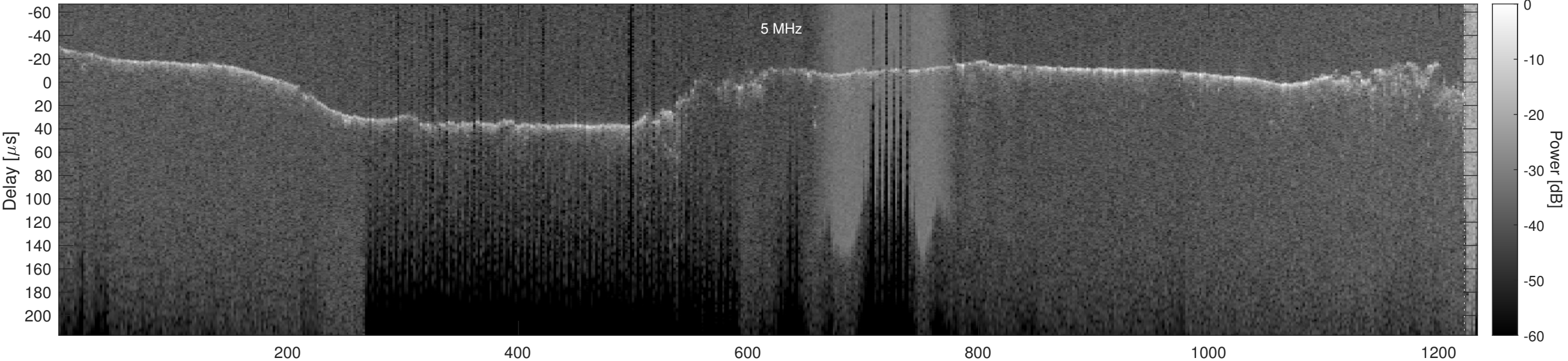
Orbit 4199, Optimized, Window, Channel 2
