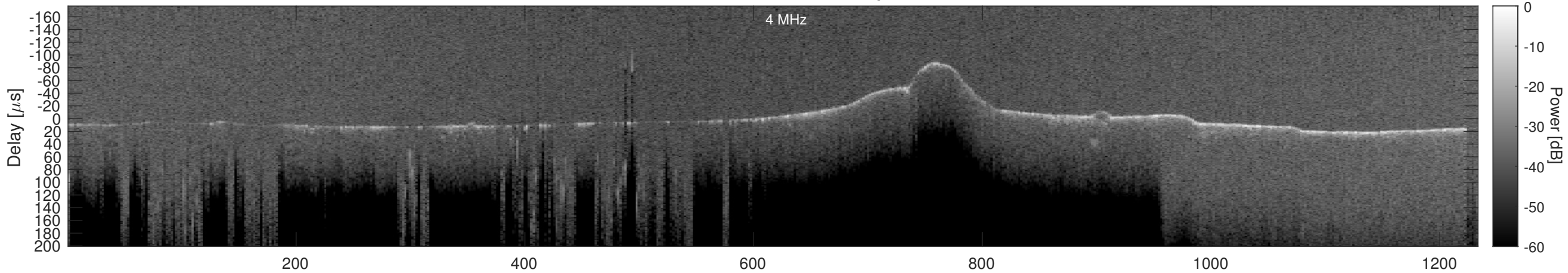
Orbit 4201, Cluttergram
