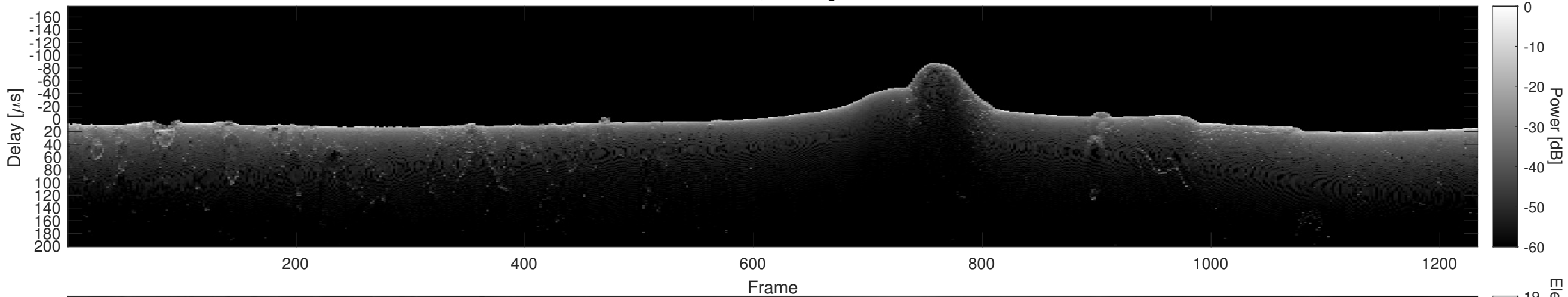
Orbit 4201, Cluttergram
