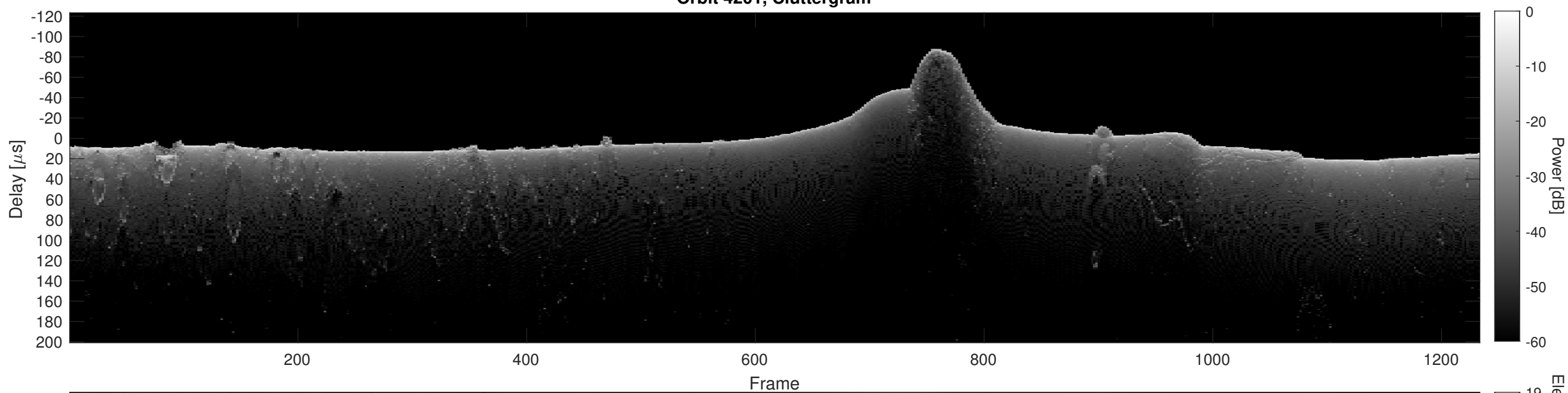
Orbit 4201, Cluttergram
