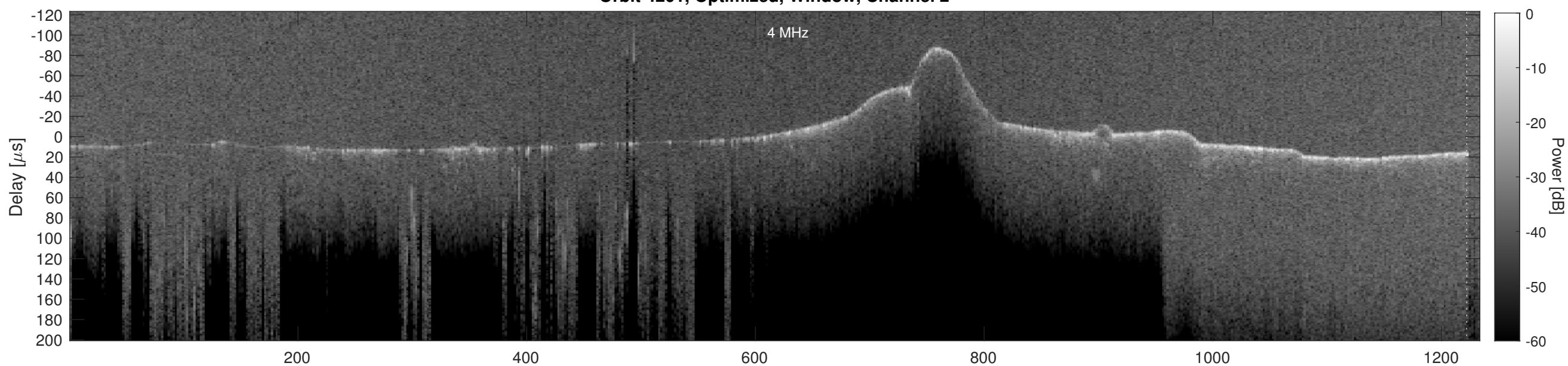
Orbit 4201, Cluttergram
