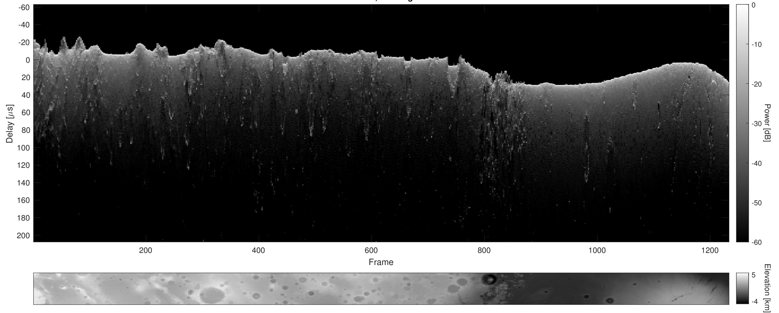
Orbit 4202, Cluttergram
