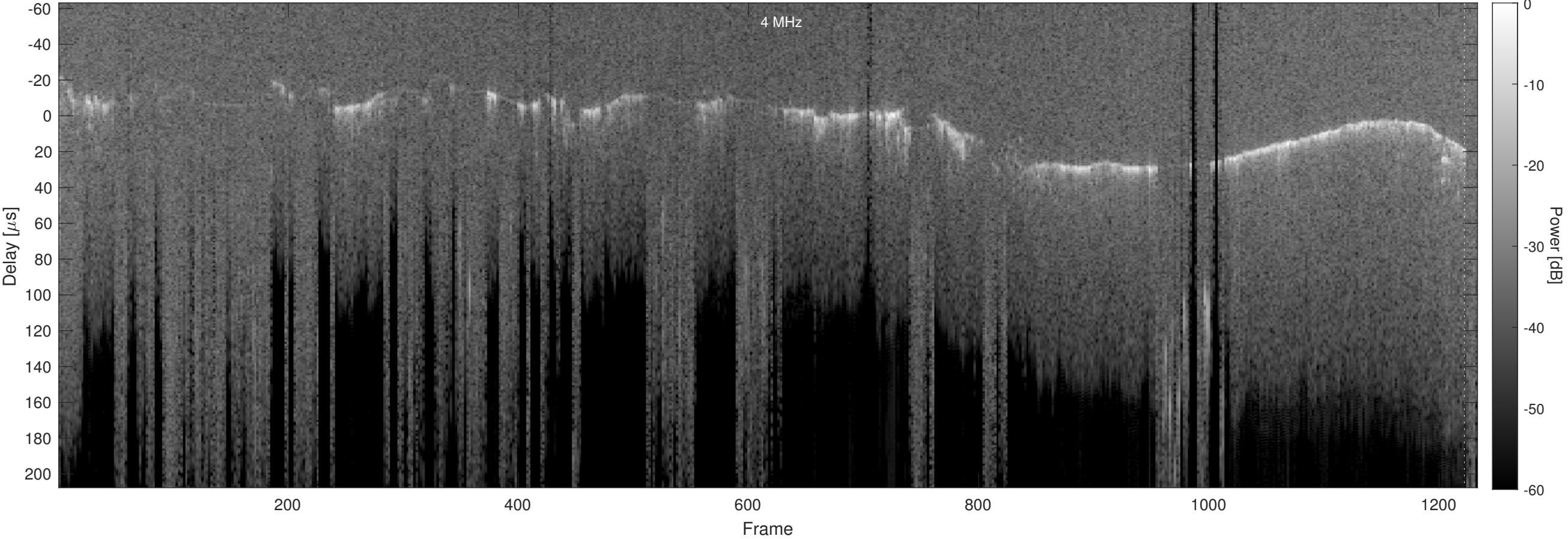
Orbit 4202, Optimized, No Window, Channel 2
