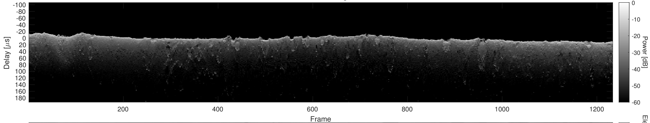
Orbit 4203, Cluttergram
