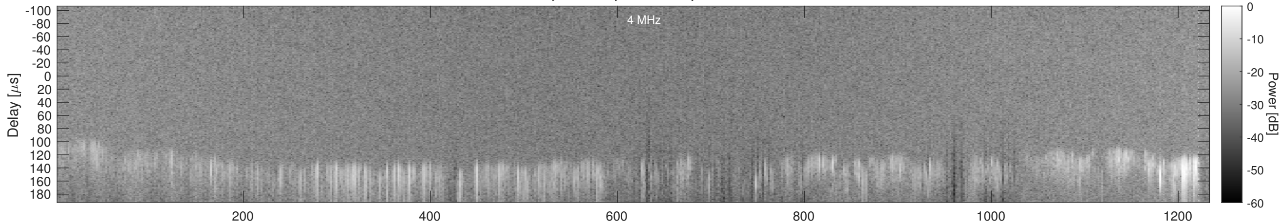
Orbit 4203, Window, Channel 2, Chapman
