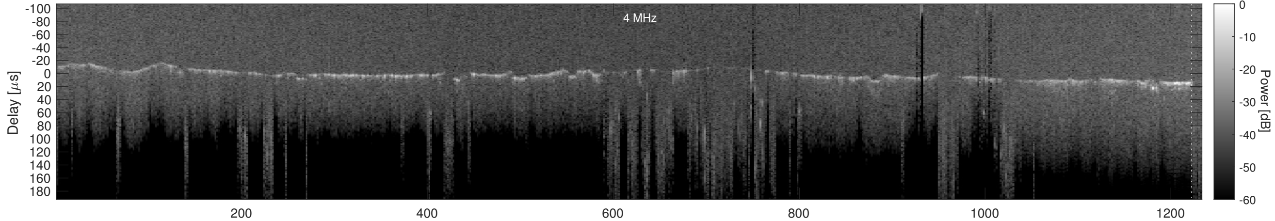
Orbit 4203, Cluttergram
