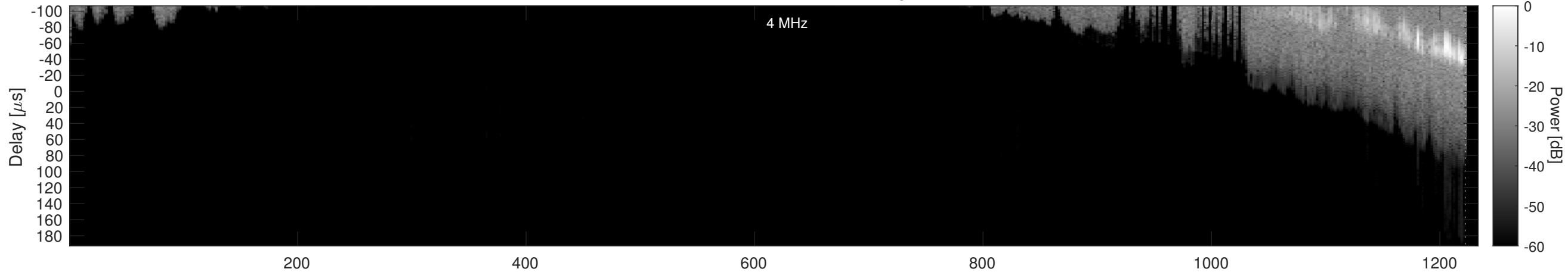
Orbit 4203, Window, Channel 2, Optimized
